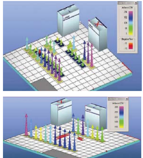
Figure 2. Computational Fluid Dynamics is a simulation tool designed to demonstrate the air flow characteristics of a raised floor. CFD provides a better understanding of why hot spots are present and the effects of under floor obstructions on air flow.
